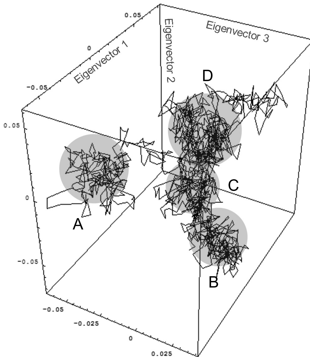
Figure 4.12 - Plot of first three backbone right singular vectors for the 1.0 ns molecular dynamics simulation of aldose reductase. These correspond to the projection of the original molecular dynamics trajectory on the three dominant eigenvectors. Protein conformational substates are highlighted using shaded circles and labeled from A to D.
