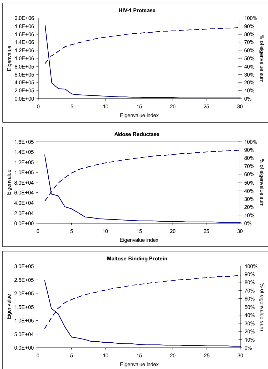
Figure 4.16 - Eigenvalues (continuous line) and percentage of eigenvalue sum (broken line) for the binding site PCA analysis of the molecular dynamics trajectories.
