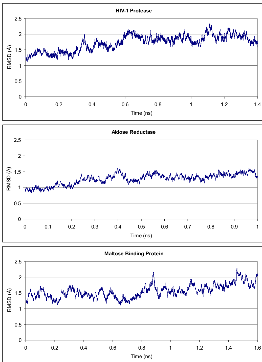
Figure 4.2 – \alpha -Carbon RMSD progression for the molecular dynamics simulations of the three model systems.
