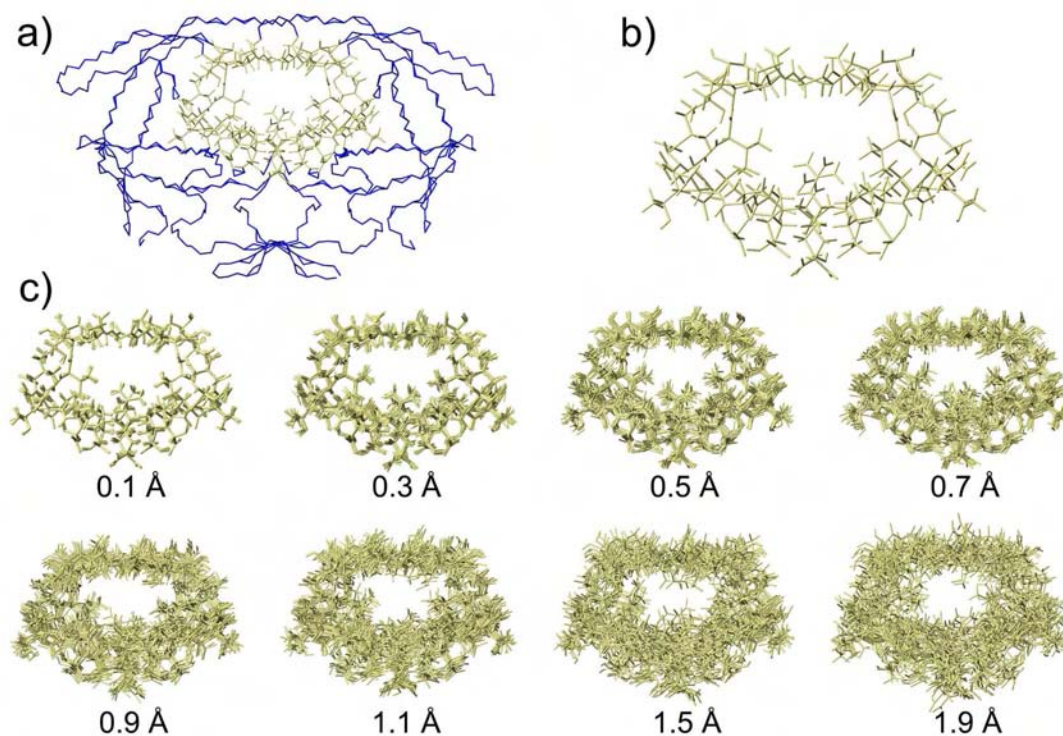
Figure 3.1 - Conformational sampling of binding site conformations. a) The experimentally determined structure of the model proteins (HIV-1 protease shown) was used as a starting point for a high temperature molecular dynamics simulation. The entire protein backbone is shown in blue and the residues defining the shape of the binding site are highlighted in yellow. In b) we show a magnified view of the binding site displaying only the residues used for the RMSD calculations. c) The multiple conformational snapshots resulting from the sampling simulations were sorted and grouped according to the RMSD to the original experimental structure. In c) we show the superposition of 10 representative structures for eight different similarity groups. Structures from these groups were subsequently used for docking as representatives of different levels of conformational flexibility.
