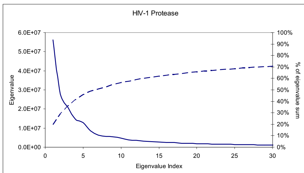
Figure 4.20 - Eigenvalues (continuous line) and percentage of eigenvalue sum (broken line) for the all-atom PCA analysis of the molecular dynamics trajectory for HIV-1 protease.
