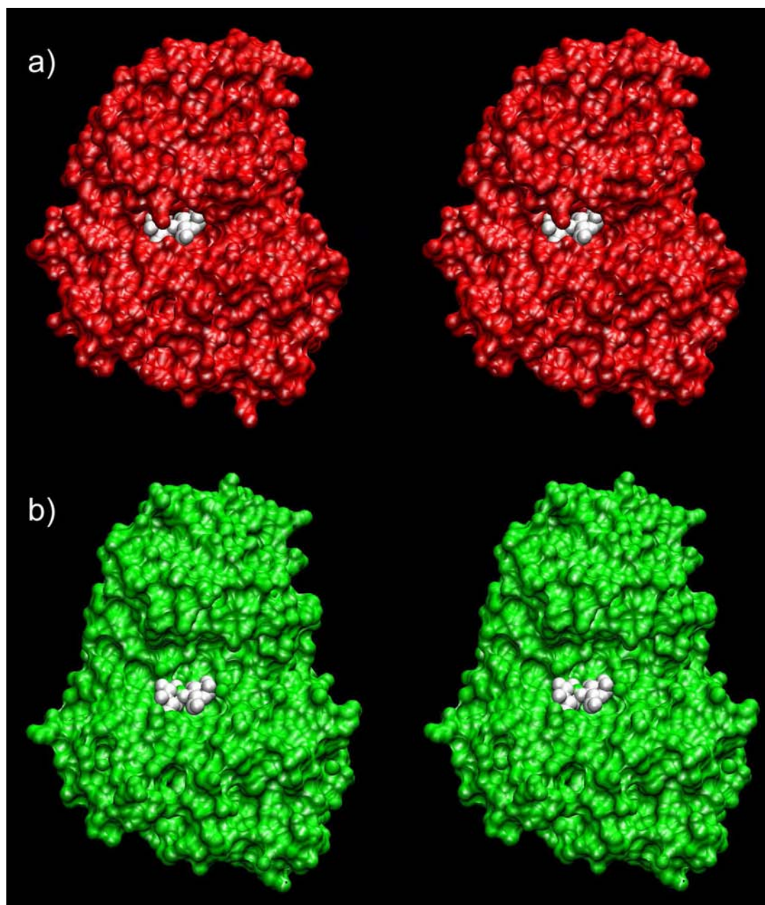
Figure A.8 – Surface representation for the a) bound and b) unbound forms of maltose binding protein (the ligand is shown in the unbound form for comparison purposes). After binding maltose the two domains close around a hinge in the center of the protein and change the solvent exposure of the binding site.
