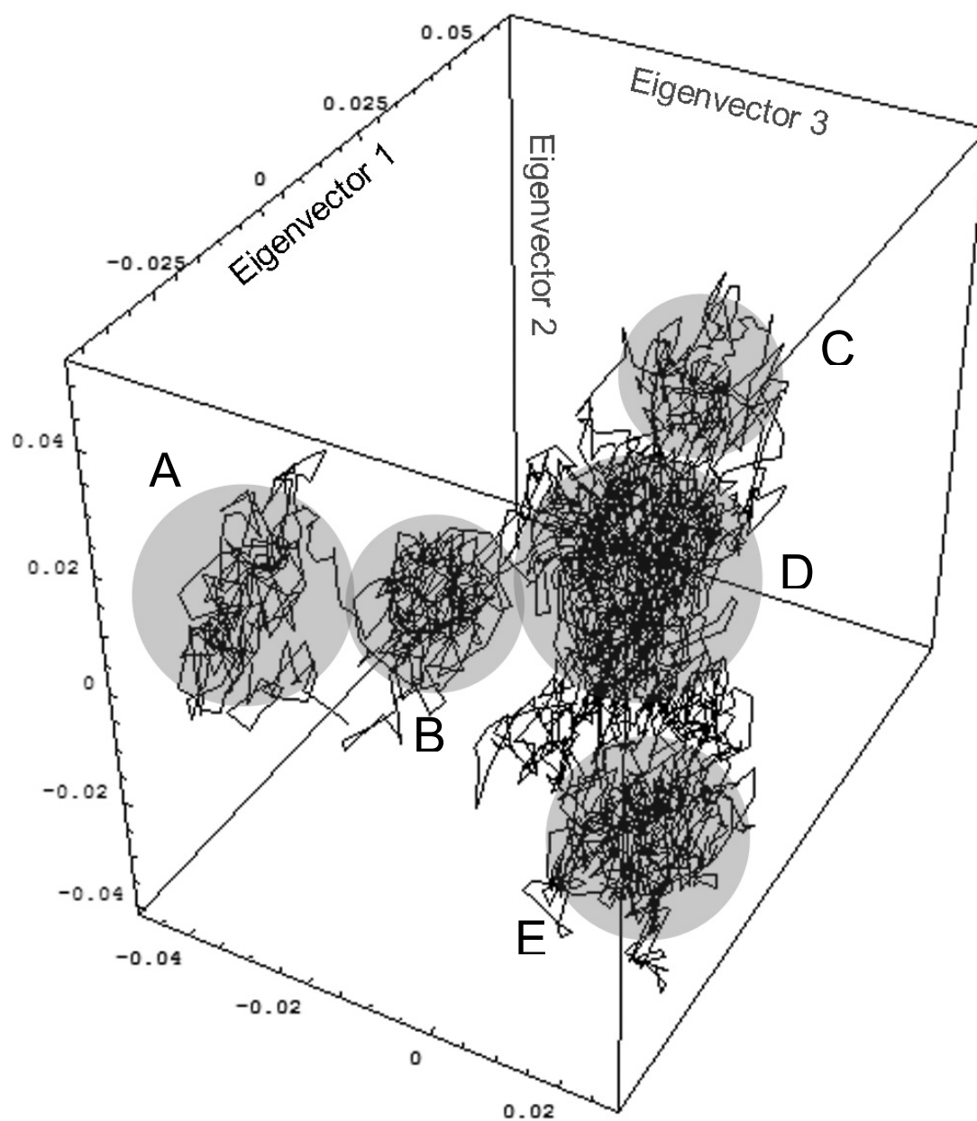
Figure 4.10 – Plot of first three backbone right singular vectors for the 1.4 ns molecular dynamics simulation of HIV-1 protease. These correspond to the projection of the original molecular dynamics trajectory on the three dominant eigenvectors. Protein conformational substates are highlighted using shaded circles and labeled from A to E.
