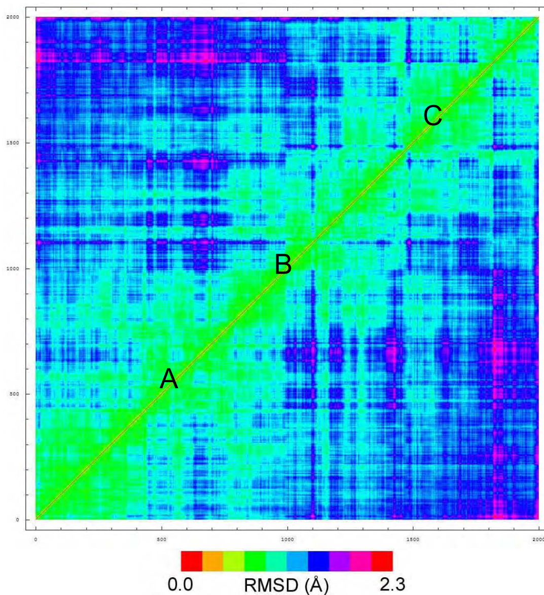
Figure 4.15 - Backbone RMSD matrix for the 1.6 ns molecular dynamics simulation of maltose binding protein. The two axis represent 2000 backbone structures sampled every 8 ps. The RMSD value between two structures is represented off the diagonal at the intersection of the respective indices (note: the data on the two side of the diagonal is identical). Protein conformational substates identified using Figure 4.14 are labeled from A to C.
