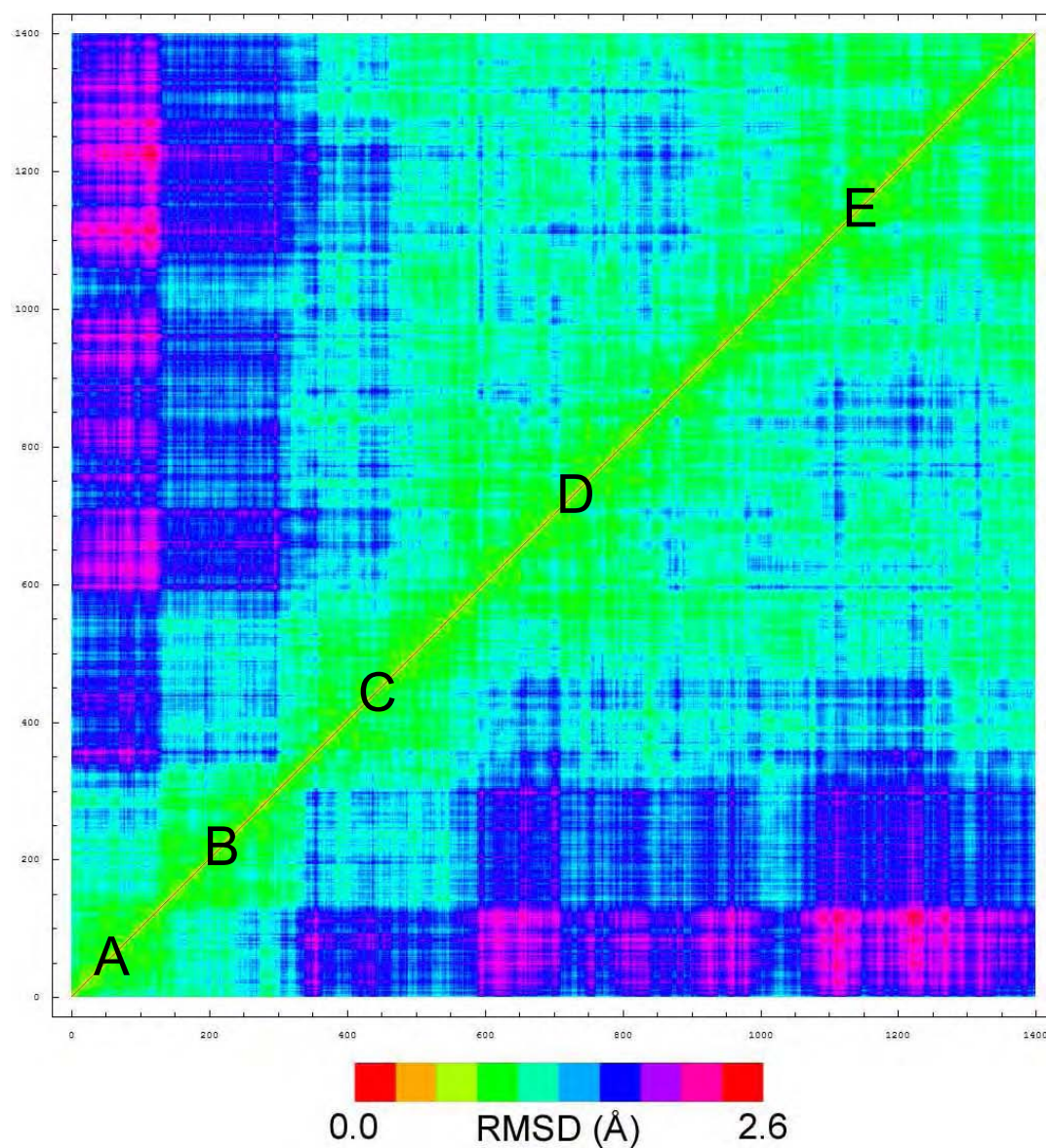
Figure 4.11 – Backbone RMSD matrix for the 1.4 ns molecular dynamics simulation of HIV-1 protease. The two axis represent 1400 backbone structures sampled every 10 ps. The RMSD value between two structures is represented off the diagonal at the intersection of the respective indices (note: the data on the two side of the diagonal is identical). Protein conformational substates identified using Figure 4.10 are labeled from A to E.
