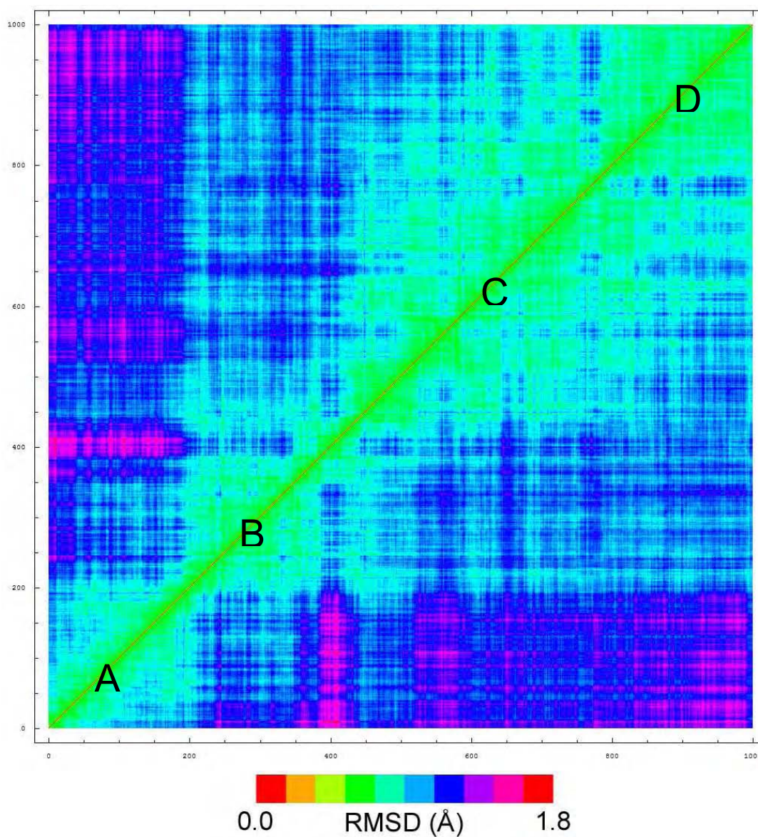
Figure 4.13 - Backbone RMSD matrix for the 1.0 ns molecular dynamics simulation of aldose reductase. The two axis represent 1000 backbone structures sampled every 10 ps. The RMSD value between two structures is represented off the diagonal at the intersection of the respective indices (note: the data on the two side of the diagonal is identical). Protein conformational substates identified using Figure 4.12 are labeled from A to D.
