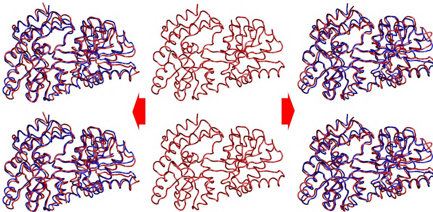
Figure 4.8 – Stereoview of the first mode of motion for the backbone of maltose binding protein. The motion shown is for the red representation. The blue representation is fixed and is used as a reference for visualization of the motion. The figures and should be viewed in portrait mode by looking up and down to give the illusion of motion. The center representation corresponds to the experimental conformation. The top and bottom views represent alternative conformations for the protein as it moves in opposite directions along the first mode of motion.
