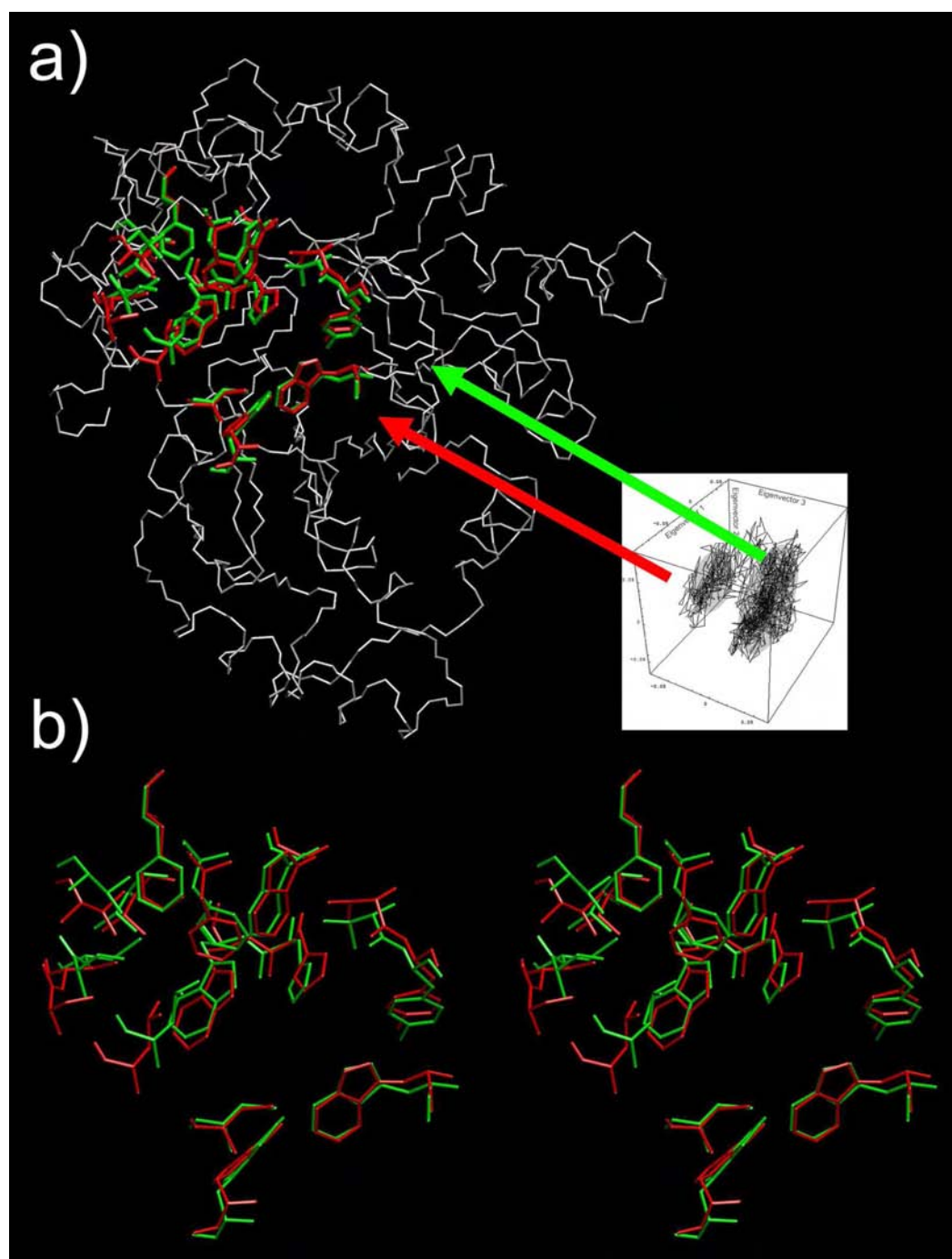
Figure 5.3 – Identification of representative conformations for the binding site of aldose reductase. a) Two conformations were identified using the right singular vectors (top right, see also Figure 4.18). b) Magnified stereoview of the variable binding site region.
