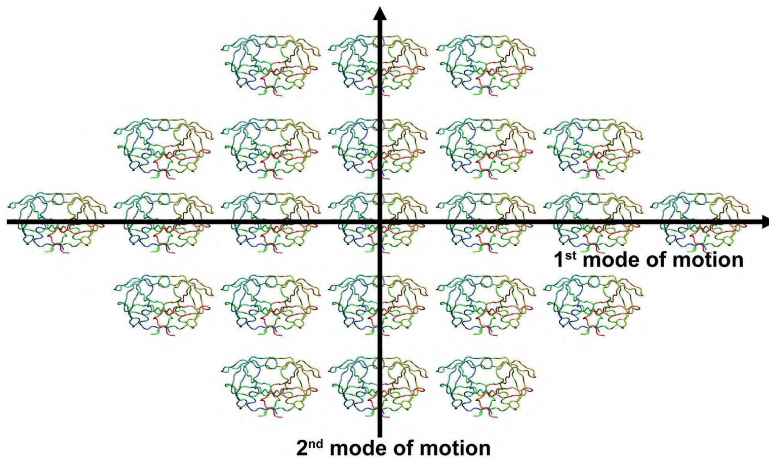
Figure 5.1 - A grid of structure representing the protein flexibility can be generated by sampling along the first two modes of motion.
