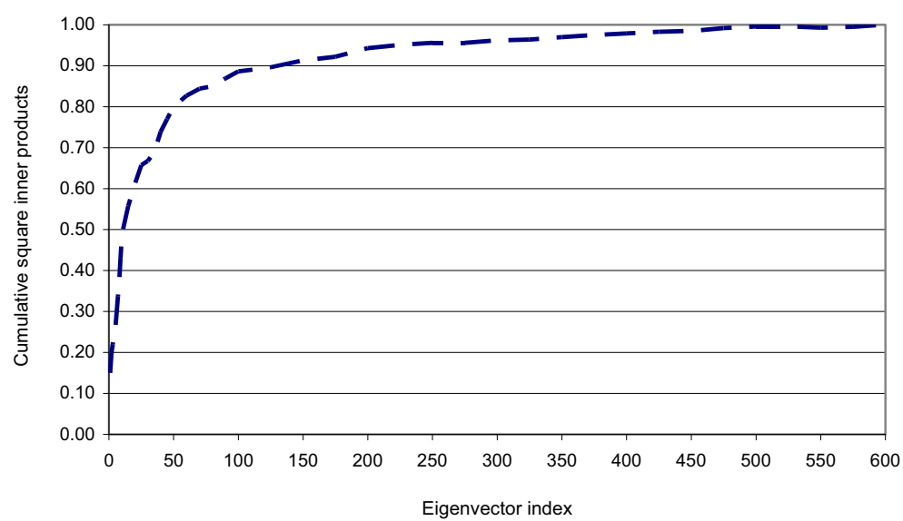
Figure 4.22 - Cumulative inner products from the projection of the molecular dynamics eigenvectors onto the first three eigenvectors derived from experimental data for HIV-1 protease.
