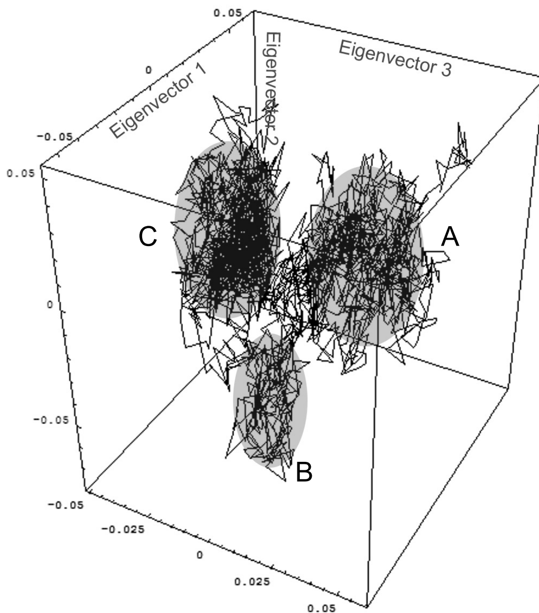
Figure 4.19 - Plot of first three binding site right singular vectors for the 1.6 ns molecular dynamics simulation of maltose binding protein. These correspond to the projection of the original molecular dynamics trajectory on the three dominant eigenvectors. Protein conformational substates are highlighted using shaded circles and labeled from A to C.
