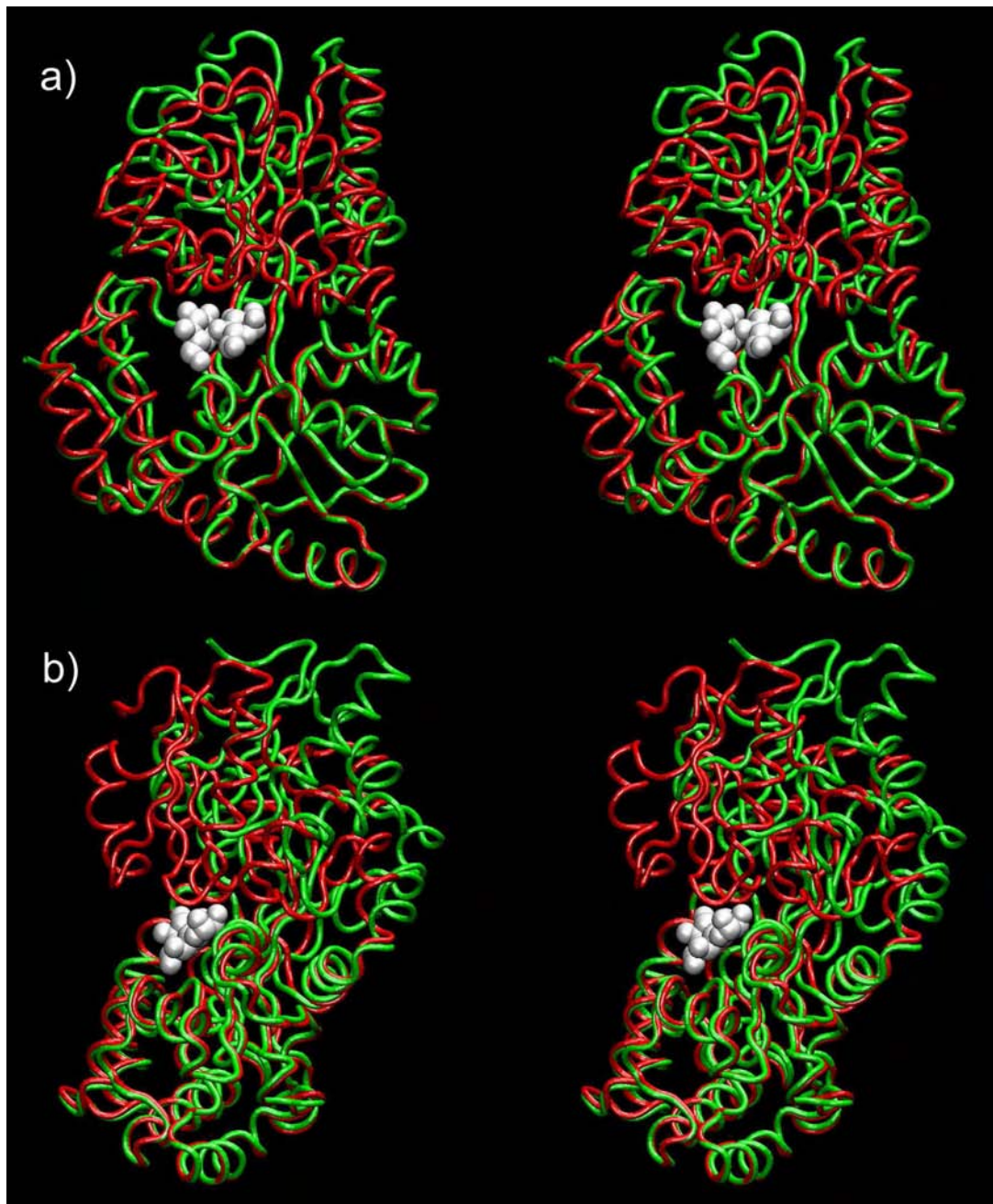
Figure A.7 – a) Front and b) side stereoviews of maltose binding protein. The bound form is shown in red and the unbound form in green. The position of the ligand for the bound structure is shown using the sphere model (white). When the protein binds the ligand the structure bends around an hinge point situated approximately in the center of the protein.
