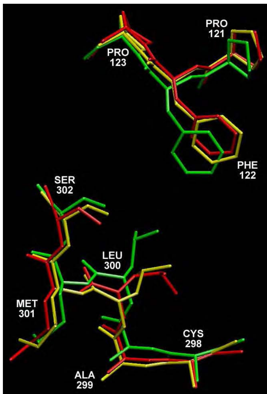
Figure 5.9 - Approximation (yellow) of the binding site bound conformation (red) of aldose reductase using the unbound conformation (green) as a starting point and searching along 40 main modes of collective motion.
