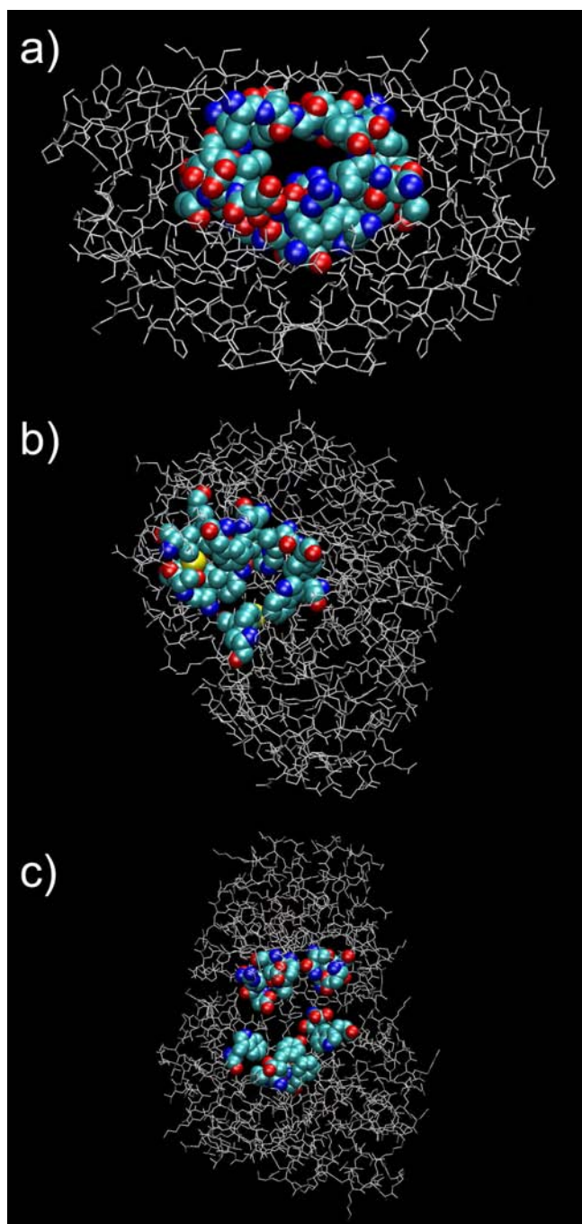
Figure 4.1 – Binding site atoms used for PCA. The atoms used for the PCA calculation are shown using VDW representation for a) HIV-1 protease, b) aldose reductase, and c) maltose binding protein.
