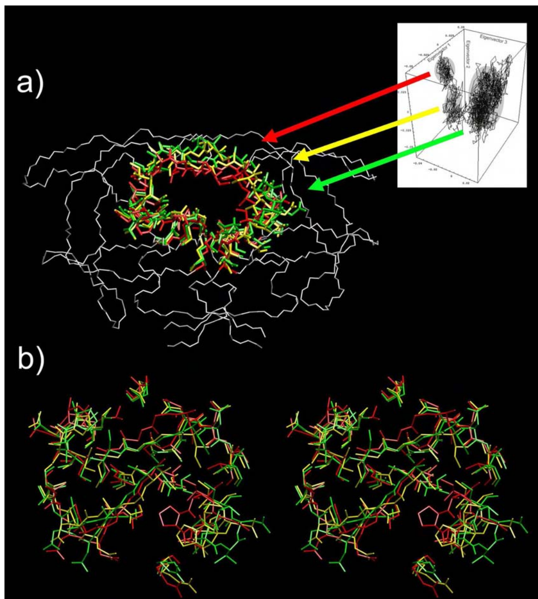
Figure 5.2 – Identification of representative conformations for the binding site of HIV-1 protease. a) Representative conformations for the three conformational substates were identified from the right singular vectors of a molecular dynamics simulation (top right, see also Figure 4.17). The heavy atom positions for the variable regions are shown in red, yellow, and green. The remaining backbone of the protein is shown in white. b) Magnified stereoview of the variable binding site region (note: image is rotated 90° forward relative to the view in a) ).
