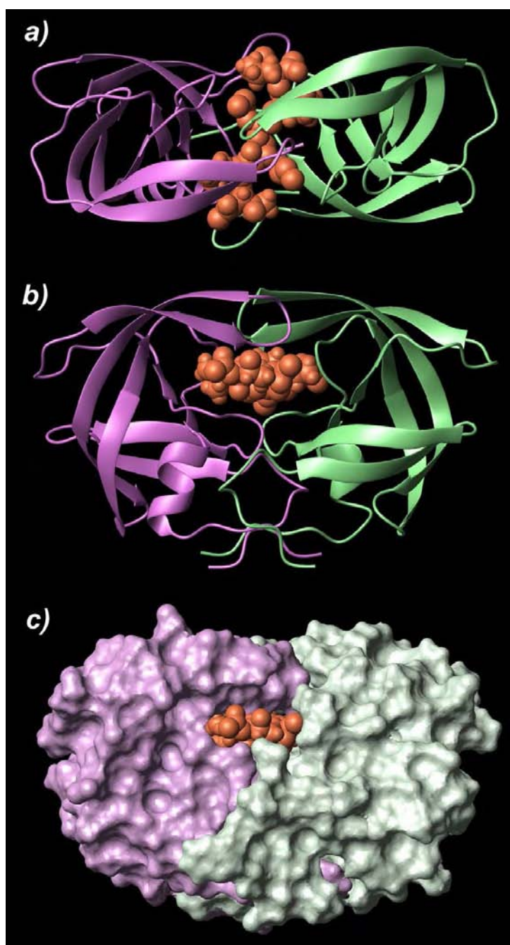
Figure A.1 - 3D structure of HIV-1 protease homodimer complexed with an inhibitor. On the a) top view and b) side view the \beta -hairpin flaps wrapping around the ligand are shown. c) in a space filling view the tight fit of the ligand in the binding site is shown indicating the need for a protein motion to allow for ligand entry and exit.
