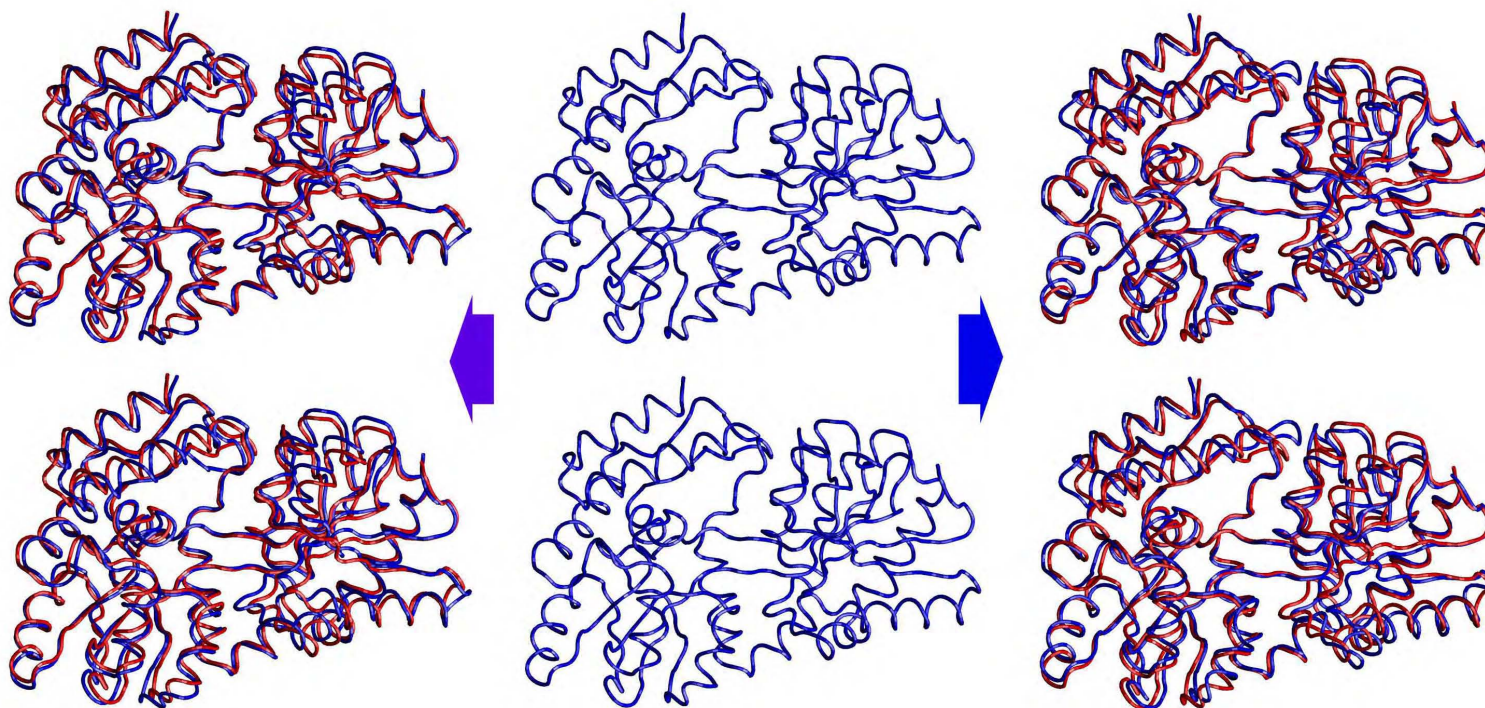
Figure 4.9 — Stereoview of the second mode of motion for the backbone of maltose binding protein. The motion shown is for the blue representation. The red representation is fixed and is used as a reference for visualization of the motion. The figures should be viewed in portrait mode by looking up and down to give the illusion of motion. The center representation corresponds to the experimental conformation. The top and bottom views represent alternative conformations for the protein as it moves in opposite directions along the second mode of motion.
