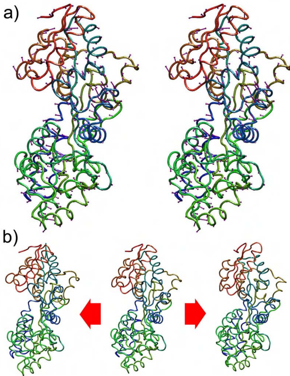
Figure 4.7 - First mode of motion for the backbone of maltose binding protein. a) Stereoview of the mapping of the first eigenvector on the C- \alpha atoms. b) Changes in conformation corresponding to a motion in both directions along the first mode of motion starting from the experimental structure (center).
