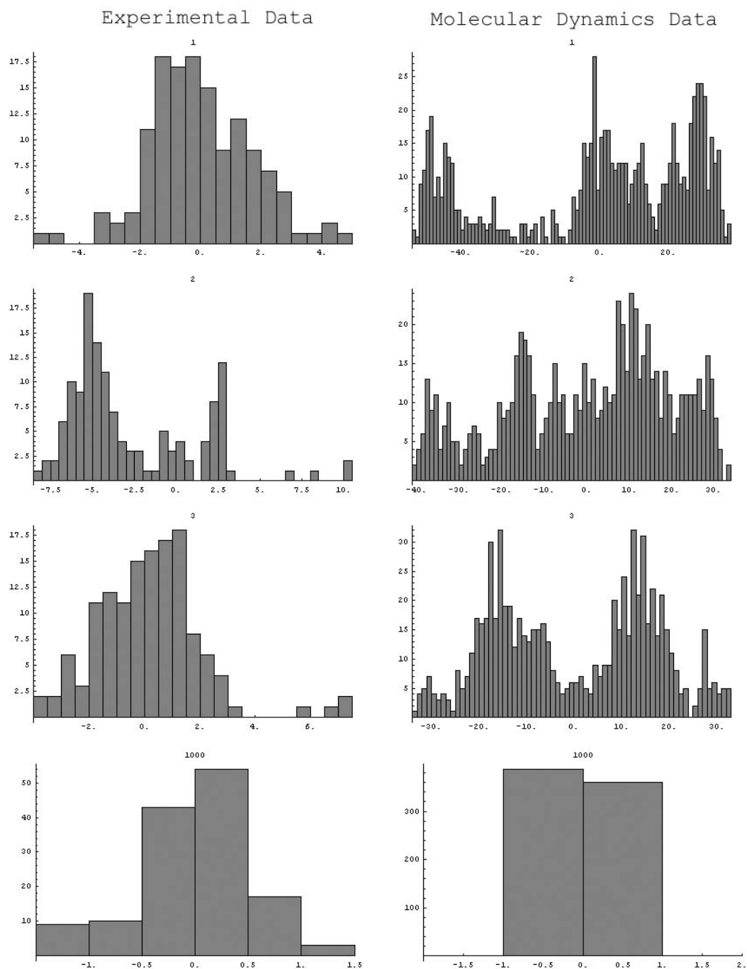
Figure 4.24 - Histogram analysis comparison of the 1 st , 2 nd , 3 rd , and 1000 th right singular vectors for the experimental and MD data.
