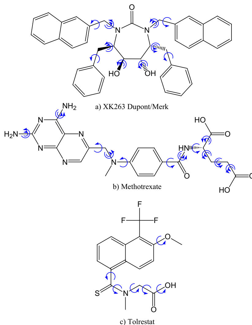
Figure 3.2 - Ligands and degrees of freedom used in docking. For the case of rigid ligand docking all torsional degrees of freedom were set to the values found in the experimental structure. For the case of flexible ligand docking the arrows indicate the torsional degrees of freedom allowed to vary during the flexible ligand conformational search. In cases a) and b) where more than one level of conformational flexibility was explored, the bonds labeled with the single arrows indicate the degrees of freedom searched in the least flexible model and the bonds labeled with double arrows indicate the degrees of freedom that were added for the most flexible model.
