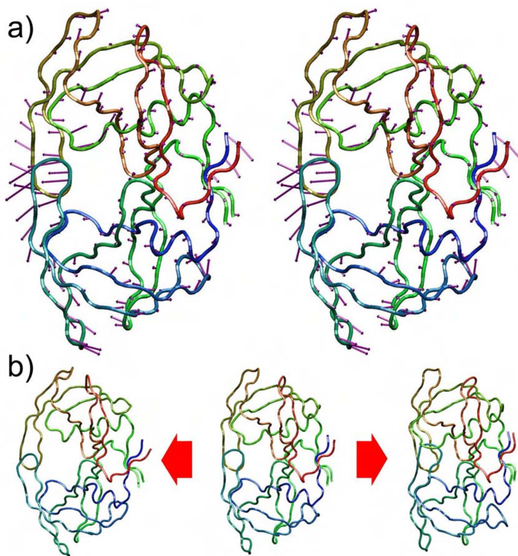
Figure 4.4 – First mode of motion for the backbone of HIV-1 protease. The backbone is colored from red to blue as a function of the residue number. a) Stereoview of the mapping of the first eigenvector on the C- \alpha atoms. The directions of motions are indicated by purple arrows. b) Changes in conformation corresponding to a motion in both directions along the first mode of motion starting from the experimental structure (center).
