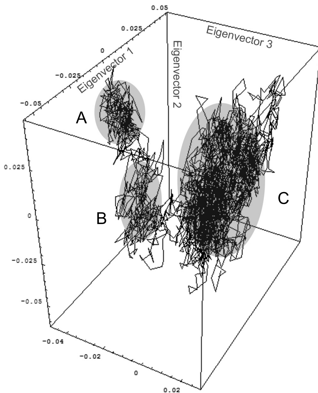
Figure 4.17 - Plot of first three binding site right singular vectors for the 1.4 ns molecular dynamics simulation of HIV-1 protease. These correspond to the projection of the original molecular dynamics trajectory on the three dominant eigenvectors. Protein conformational substates are highlighted using shaded circles and labeled from A to C.
