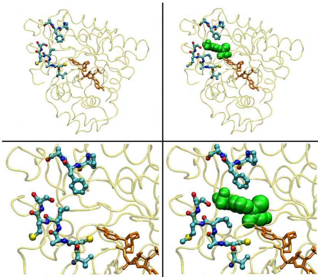
Figure A.4 – Binding site comparison for the unbound and bound forms of aldose reductase. The unbound form of aldose reductase is shown on the left and the bound form is shown on the right. The bottom figures zoom in the corresponding top figures to show aminoacids whose rearrangements open a pocket that make the binding possible. The cofactor NADPH is shown in orange.
