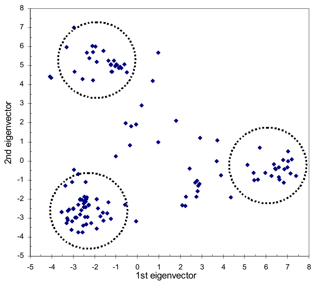
Figure 4.21 - Projection of coordinate vectors of 135 experimental HIV-1 protease structures on the plane defined by the two dominant eigenvectors of the PCA. The circles indicate clustering of structures in the essential subspace.
