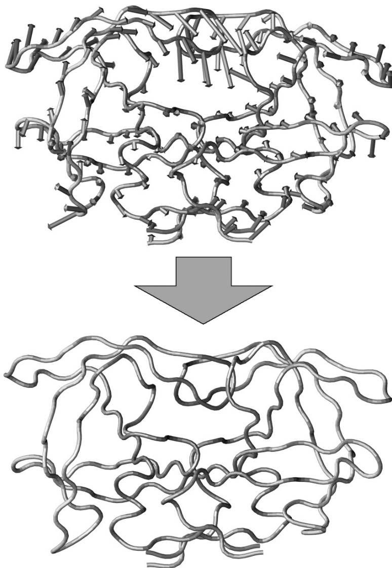
Figure 2.5 – Representation of a collective degree of freedom for HIV-1 protease. Full protein flexibility can be represented in a low dimensional space using collective degrees of freedom. One method to obtain these is Principal Component Analysis. Principal components correspond to a concerted motion of the protein. The first principal component for HIV-1 protease is indicated by the arrows (top). By following this collective degree of freedom it is possible to generate alternative conformations for the receptor (bottom).
