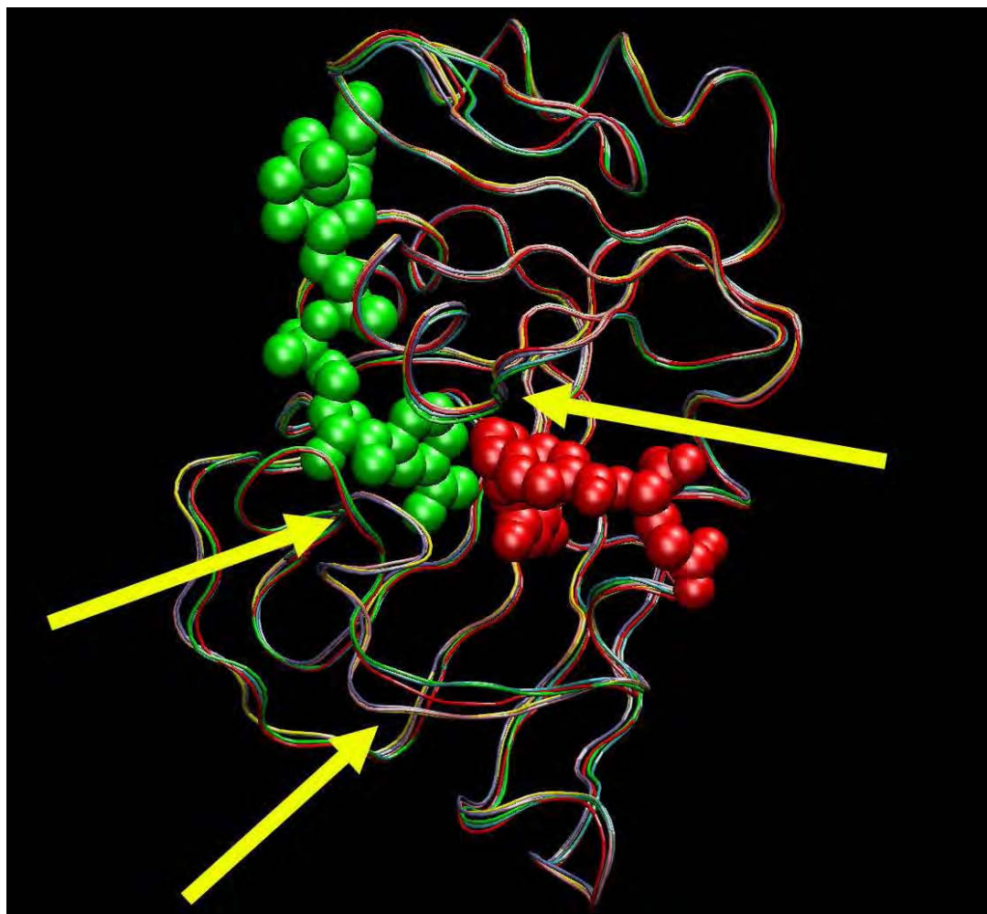
Figure A.6 – Conformational changes during the catalytic cycle of DHFR. The conformations shown in tube representation correspond to the five detectable kinetic intermediates and to the transition state. The location of the binding site is indicated by the VDW representation of NADPH (green) and folate (red). Yellow arrows indicated the regions near the binding site that display the largest amount of variation.
