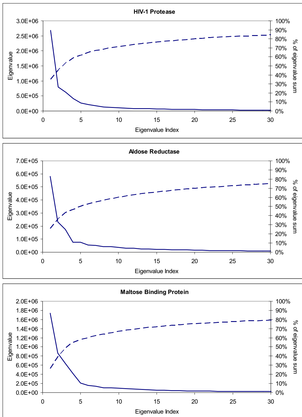
Figure 4.3 – Eigenvalues (continuous line) and percentage of eigenvalue sum (broken line) for the backbone PCA analysis of the molecular dynamics trajectories.
